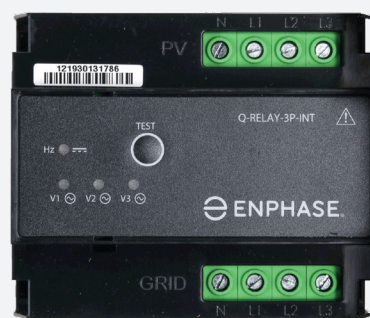
3PH 265VAC Relay Controller 84460240
